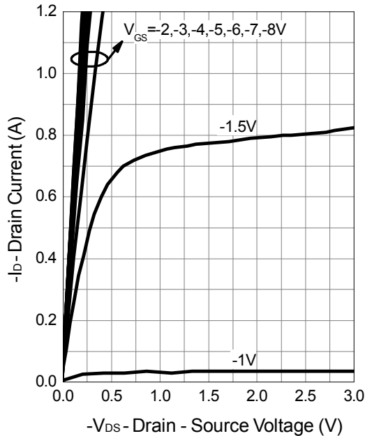
Output Characteristics
