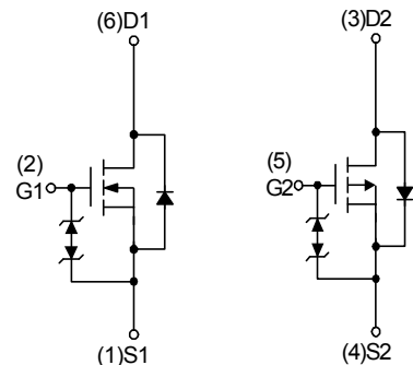
N-Channel
