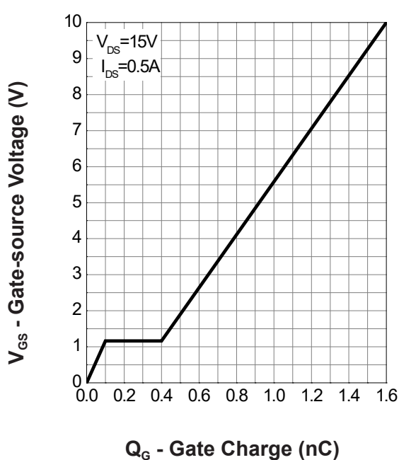
Gate Charge
